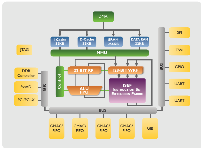
Figure 1 S5610 Block Diagram
