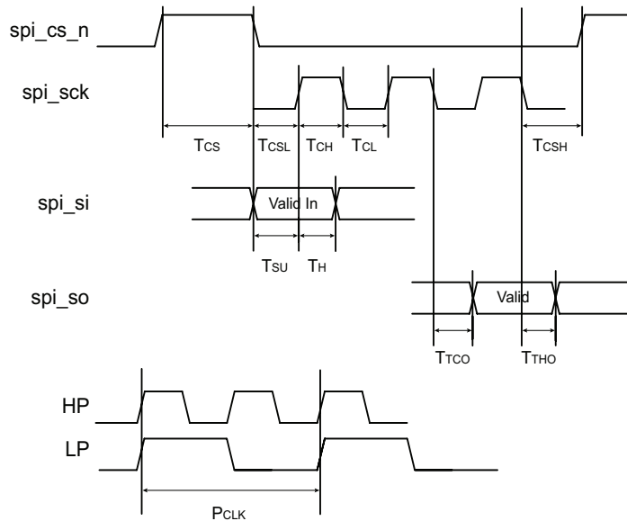
Figure 3-3 SPI timing diagram
