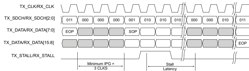
Figure 3-16 16-bit MAC-bypass timing
