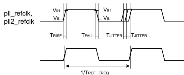
Figure 3-34 PLL timing diagram
