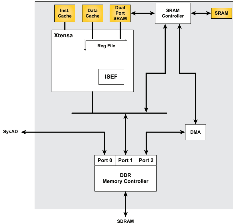
Figure 1-1 S5610 memory block diagram
