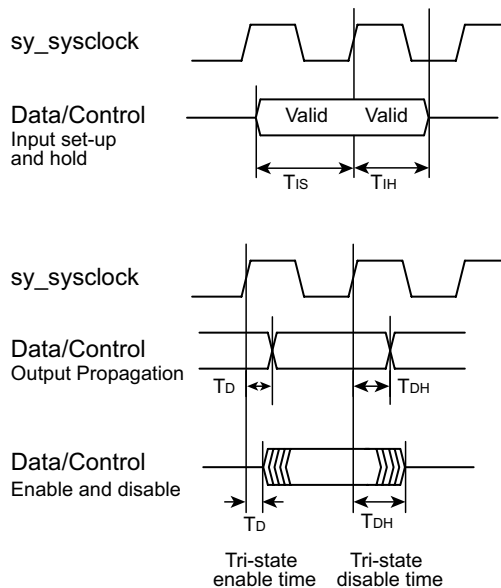
Figure 3-33 Coprocessor data and control timing diagram
