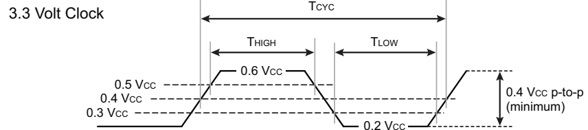
Figure 3-22 PCI clock waveform diagram
