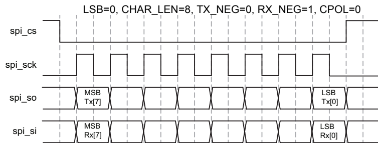
Figure 3-5 SPI timing 2
