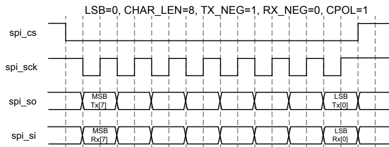
Figure 3-7 SPI timing 4
