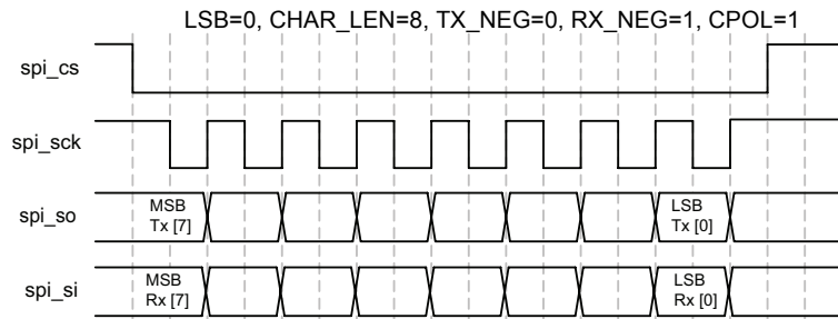
Figure 3-6 SPI timing 3
