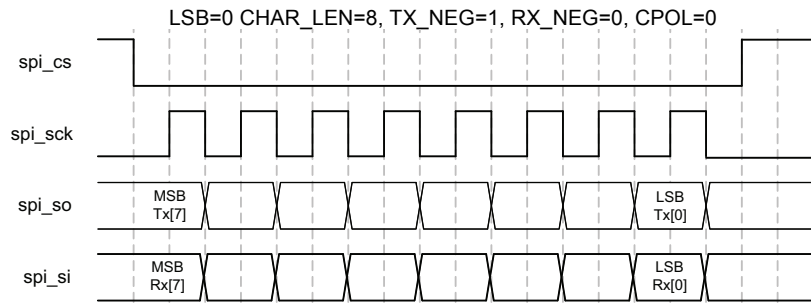
Figure 3-4 SPI timing 1
