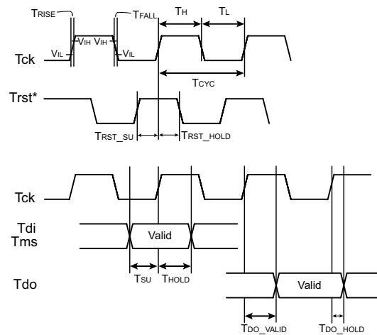
Figure 3-35 JTAG timing diagram
